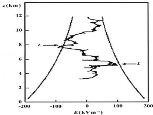
Figure 7 Balloon measurements of the electric field adapted from Marshall et al., 1995. The arrows marked L shows lightning strokes
