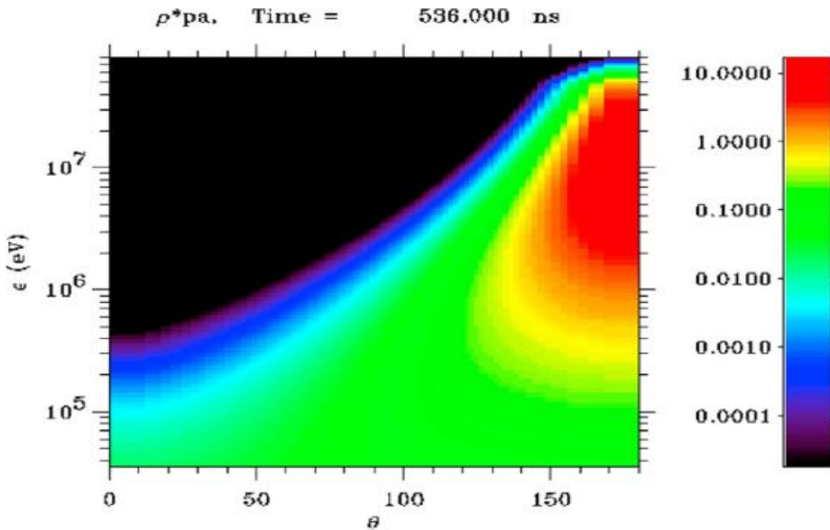
Figure 4 Electron distribution function for \delta_0 = 4 as a function of electron energy \varepsilon in eV and the angle \theta of motion of the electrons relative to the direction of the electric field.
