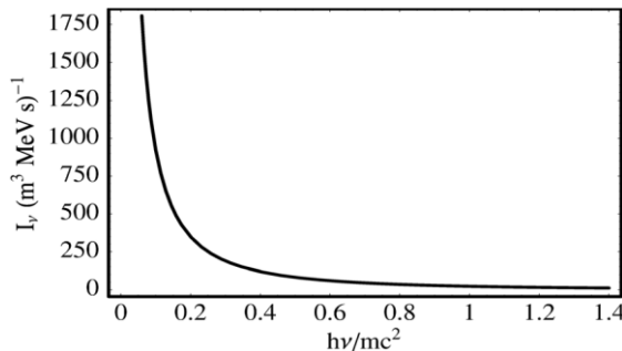
Figure 10. Model of spectral density of the bremsstrahlung emission due to RB in thundercloud at 4 km at E = 2E_c [adapted from Gurevich et al., 1999a].
