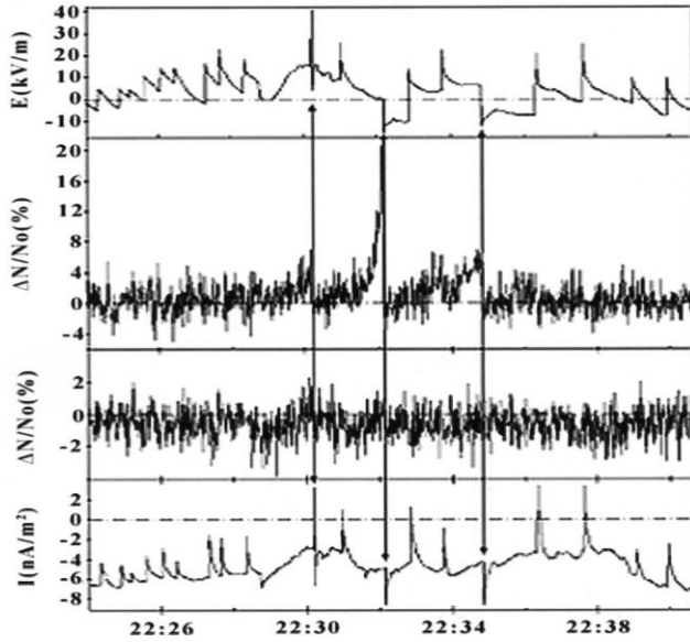
Figure 8 Observations by the Carpet air shower array at Baksan, North Caucasus during the thunderstorm on 9 July 2000. (top plate) The electric field and (second from the top) the soft component (electrons, 10–30 MeV) of cosmic rays. The arrows show lightning strokes [adapted from Alexeenko et al., 2002].
