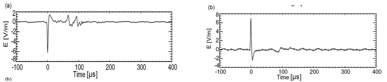
Figure 13. (a) Positive NBP and (b) negative NBP observed by Los Alamos Sferic Array adapted from Smith et al. [2002].
