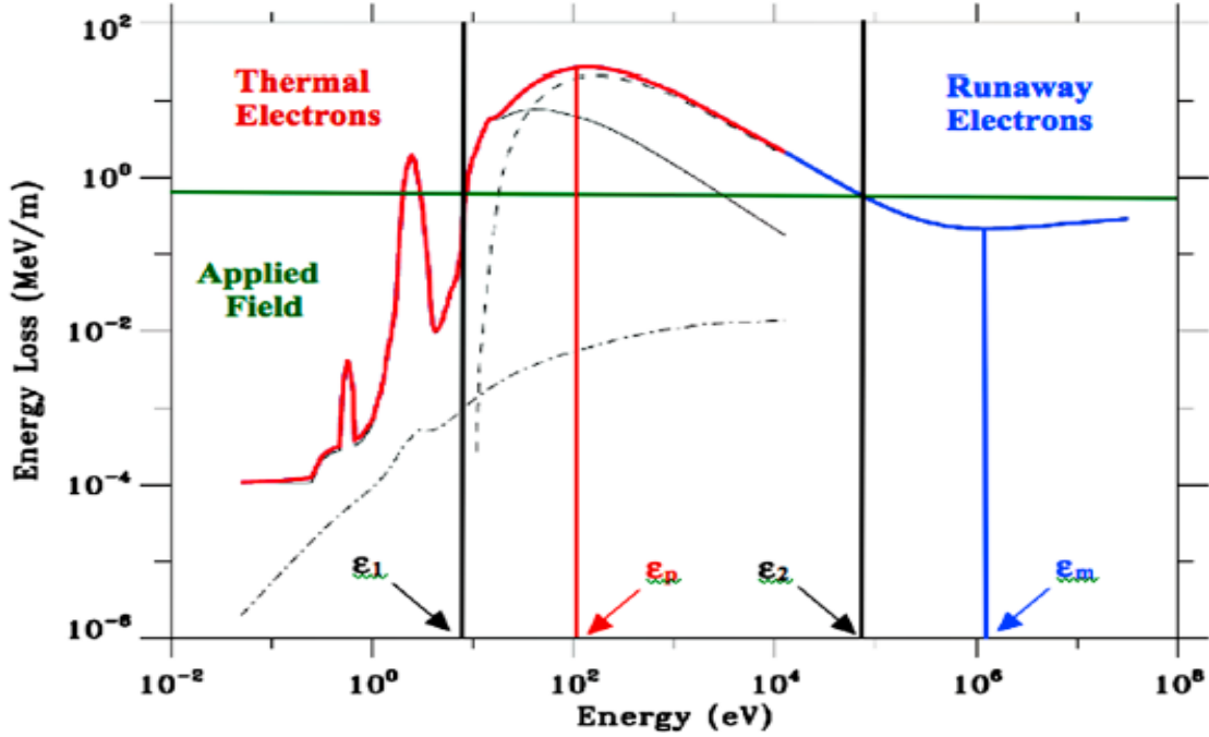
Figure 5 Energy loss rate for electrons in air as a function of electron energy. The red curve is derived from detailed cross sections for elastic, rotational, vibrational, electronic, and ionizing electron-neutral collisions in air. The solid, dashed, and dash-dotted curves represent the energy loss rate due to inelastic (sum of rotational, vibrational, and electronic processes), ionizing, and elastic collisions, respectively. The blue curve is the Bethe energy loss formula invoked at energies above 10\text{ keV} . The green line represents the magnitude of an applied electric field. \varepsilon_1 , \varepsilon_2 , \varepsilon_p , and \varepsilon_m are defined in the text.
