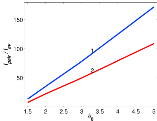
Figure 12. The ratio of the pair production length to the avalanche length as a function of \delta_0 computed for two different photon energies 10 MeV (trace 1) and 20 MeV (trace 2).
