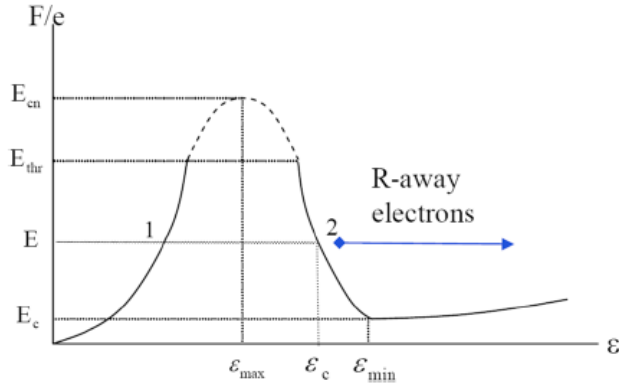
Figure 2 Schematic of the dynamical friction force in air as a function of electron energy. Traces 1 and 2 correspond to low and high energy electrons, respectively. E_{cn} is the critical field for thermal runaway, E_{th} is the breakdown threshold, and E_c is the critical field for relativistic breakdown.
