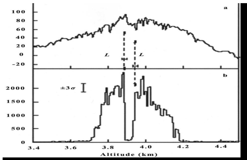
Figure 6 Balloon measurements of (top) E field and (bottom) X - rays adapted from Eack 1996
