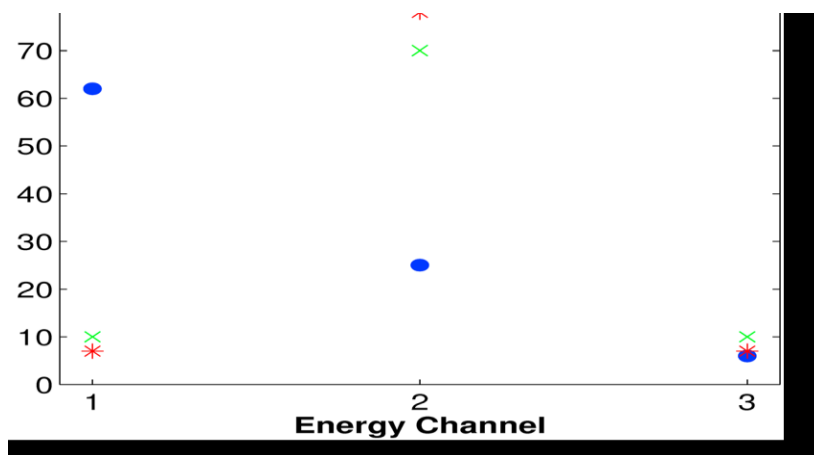
Figure 11 The computed energy spectrum for the X- ray emission given in Figure 10. The X- ray fluxes were integrated over three energy channels (30-60, 60-90, and 90-120 keV). The stars show the balloon measurements, the blue points show the spectrum at 70 m from the sources, and the crosses show the spectrum at 420 m from the source. The stars show the balloon measurements by Eack [1996]
