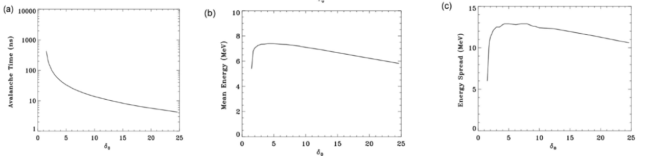
Figure 3 (a) Avalanche time in ns (b) Mean electron energy in MeV (c) Electron energy spread in MeV as a function of the over-voltage \delta_0 = E/E_c . All calculations were- performed for air at STP
