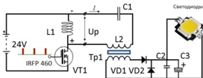
Fig. 25. The scheme of the generator
